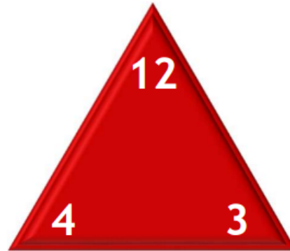
relationship triangle
