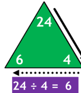
relationship triangles
